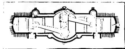
Fig. 3—Swain two-stroke cycle engine with opposed cylinders
